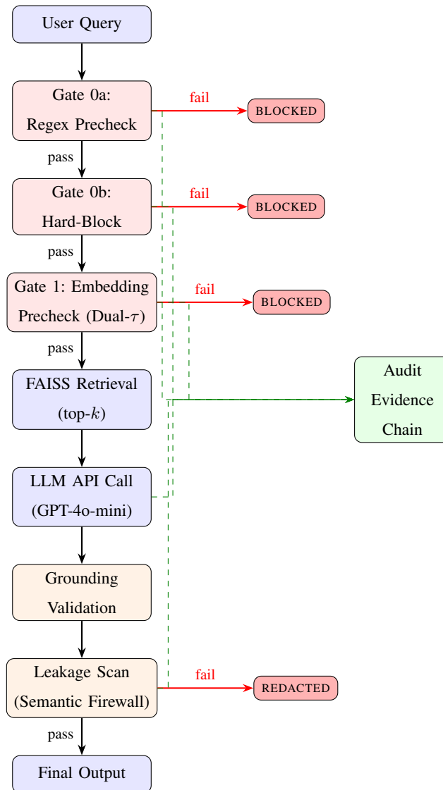
Fig. 1. SentinelFlow multi-gate pipeline architecture. Red-shaded gates are pre-LLM checks; orange-shaded are post-LLM checks. Every gate decision is logged to the tamper-evident audit chain (green, dashed). If any pre-gate fails, the LLM is never called.
